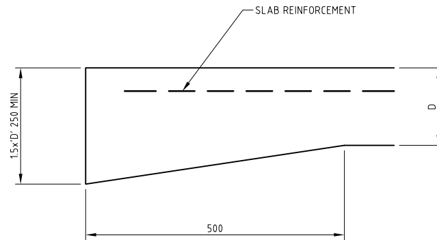
TYPICAL SECTION
